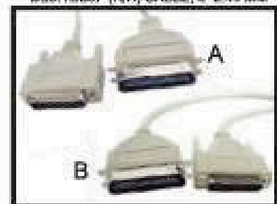
A: Q002-018-001 1.5M PRINTER CABLE DB25M/CN36M, MOLDED TYPE BEIGE, (W/ LONG SCREWS) B: Q100-019-076 1.8M IEEE 1284 CN36M/DB25M, COLOR BEIGE
