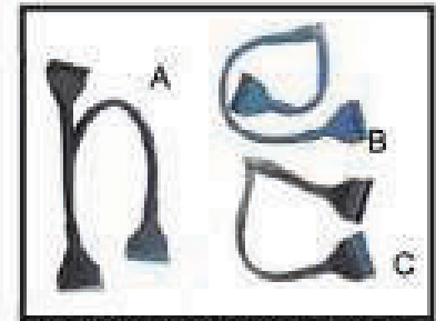
A: Q153-008-140 ATA100 FLAT CABLE 14P B: Q007-008-037 ATA100/133 HDD CABLE 40P C: Q217-008-325 ATA133 UL30276 80P*3 IDC+PULL TAB+8R JACKET BLACK
