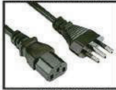
Item No. : E012018433_1.8M H05VV-F 3G 0.75MM 2 / 1.00MM 2 ,L=1.8M (SWITZERLAND APPROVAL)
